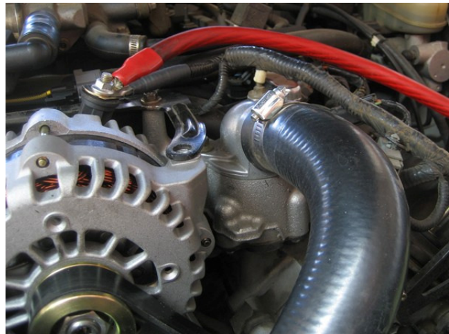
Connect the charge lead from the alternator output stud and run it to the battery positive (+). The use of aftermarket battery clamps will facilitate these connections, although ring terminals can be terminated on the cables and used to connect to OEM style clamps.
