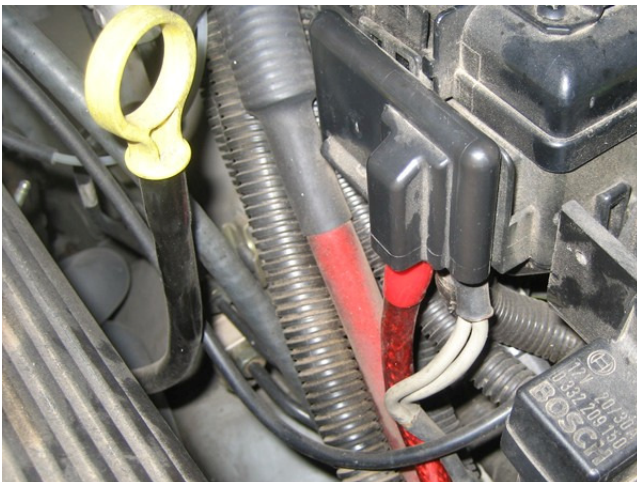
Upgrade the lead from the under hood fuse box to the battery positive (+) to a 4 AWG* cable. Note that the OEM charge lead remains in place. This may vary based on your vehicle.
